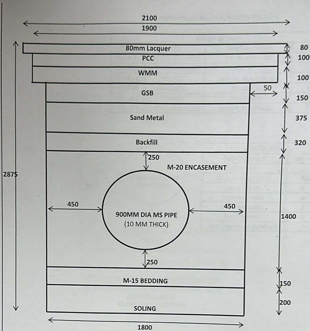
CROSS SECTION OF TRENCH FOR LAYING OF 900 MM DIA MSWM AT Maharshi Karve Road in D WARD
