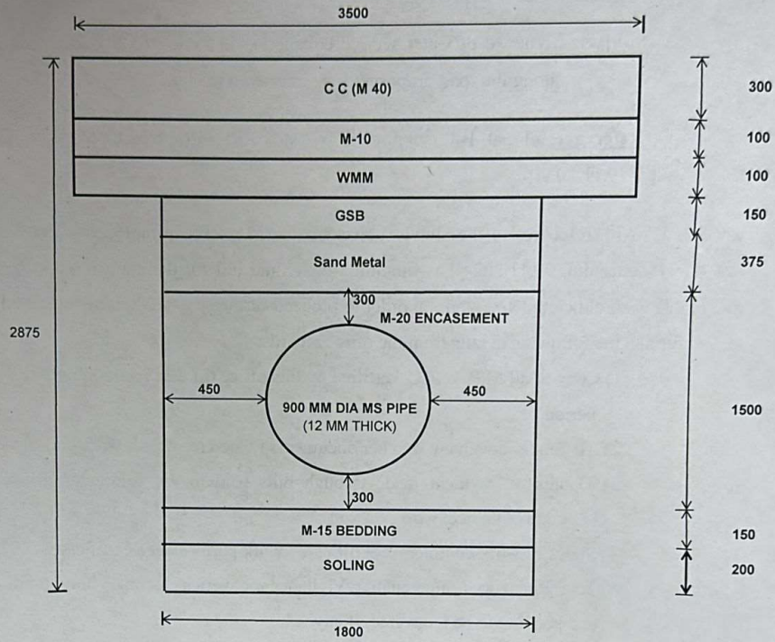
CROSS SECTION OF TRENCH FOR LAYING OF 900 MM DIA MSWM along Maharshi Karve Road in C ward (Cement Concrete Portion)
